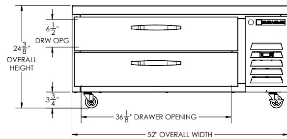
ELEVATION VIEW
